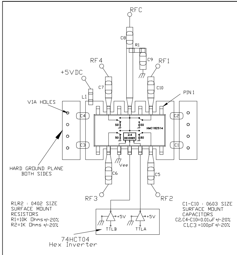
Figure 1: Floating Ground Driver for the HMC182S14 SP4T Switch.
